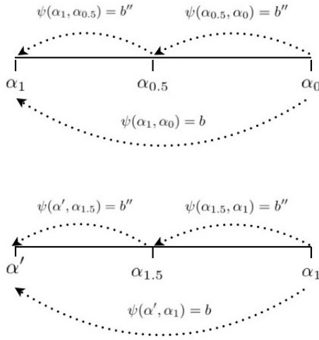
Figure 5.1: The \psi distance between outcomes
