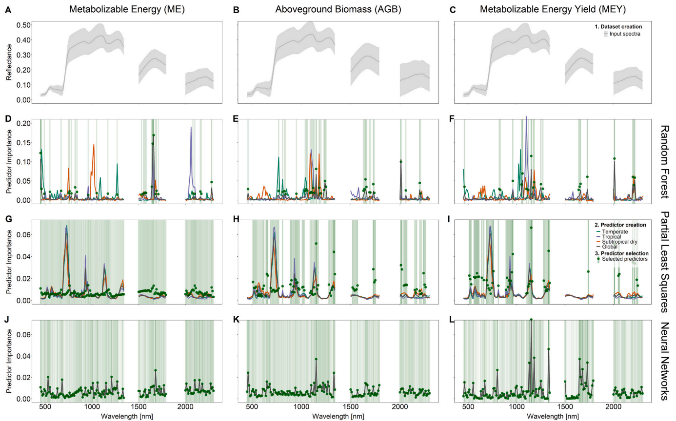
Fig. A2. Importance of single wavelengths (WL) from 450 nm to 2350 nm, using the first derivative of the canopy reflectance spectra, for predicting metabolizable energy (ME), aboveground biomass (AGB) and metabolizable energy yield (MEY) across RF regression, PLS regression, and a one-dimensional convolutional neural network. The grey line with the light grey shaded area represents the mean and standard deviation of the pure spectra input across all regions. Coloured lines indicate the importance of predictors for regional models, while black lines represent the global models. The green dots mark the final selected predictors for the prediction models and the green shading represent their relative importance in greenness intensity meaning higher importance. The white labels in the bottom graph name the spectral areas, where specific structures absorb in. The pigment area (Chlorophyll and Carotenoids) is located in the shorter wavelength area until 700 nm, the AGB area is represented between 700 and 1350 nm, while proteins absorb from 1500 nm upwards and fibre from 2000 nm in the measured spectrum. (For interpretation of the references to colour in this figure legend, the reader is referred to the web version of this article.)
