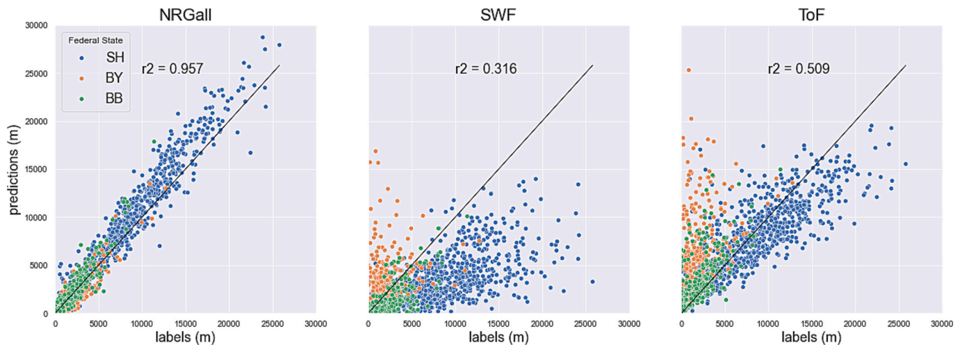
Fig. 8. Hedgerow length (m) per chip predicted vs labeled for the three products (NRGall, SWF and ToF) and three federal states (SH ( n = 825 ), BB ( n = 243 ) and BY ( n = 312 )).
