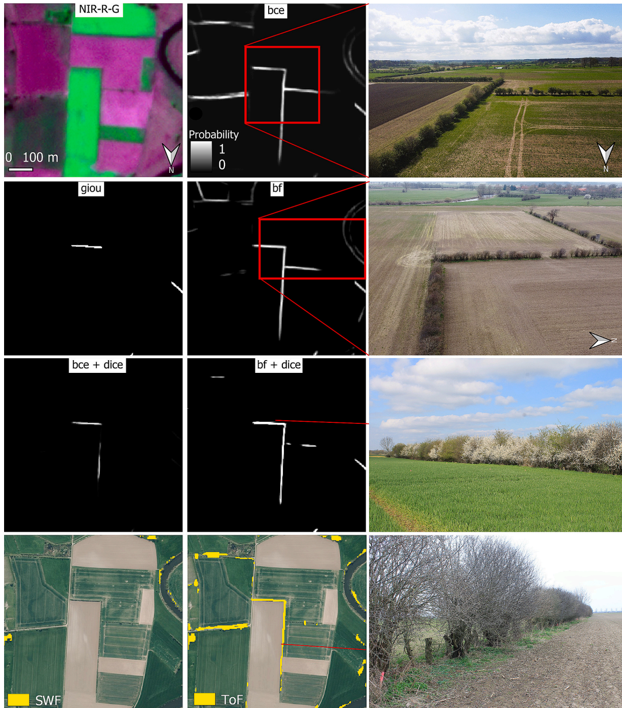
Fig. 5. Predictions with different loss functions of an example area with narrow hedgerows (2–3 m wide) (Drexler and Don, 2024). Binary crossentropy (BCE) and binary focal (BF) require a low probability threshold ( \sim 0.3 ) to correctly classify many hedgerows. The prediction probabilities of GIOU and the combinations of DICE with BF and BCE are much closer to 1 or 0. The first tile contains a PlanetScope image from August 2022 (red, near infrared and green for RGB channels). SWF and ToF are shown for comparison purposes. UAV and ground photos from winter and spring: ©Sofia Heukrodt. (EPSG: 3035, lat, lon: 3298381, 4,240,437). (For interpretation of the references to colour in this figure legend, the reader is referred to the web version of this article.)
