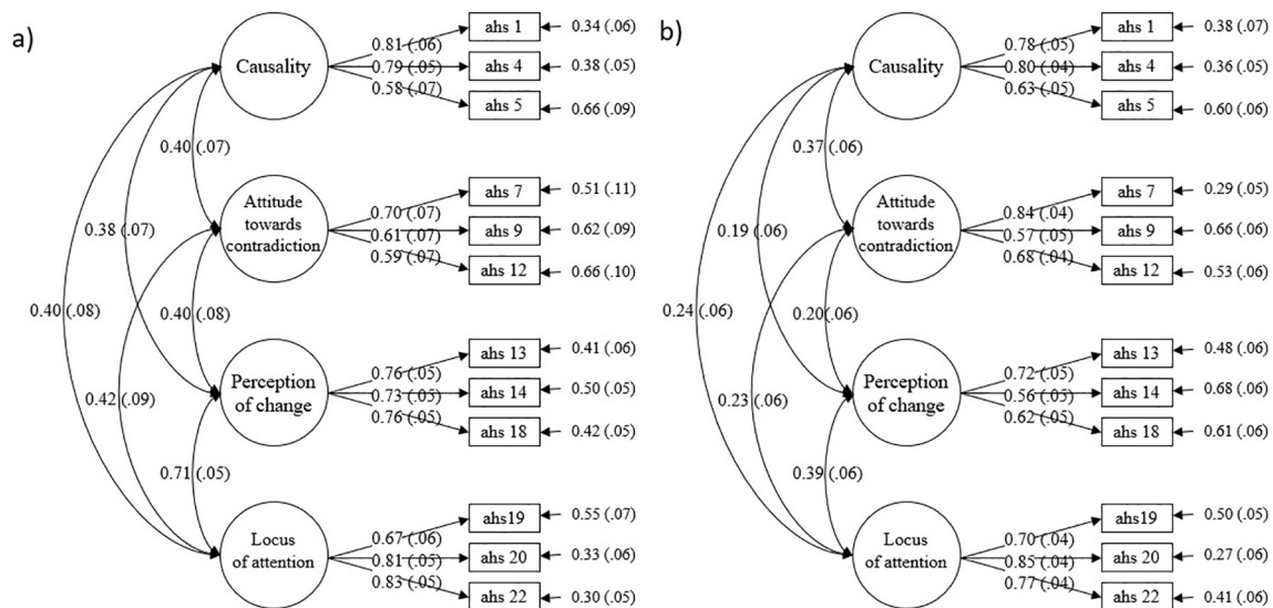
Fig. 1. Four-factor CFA models of the AHS-12.
