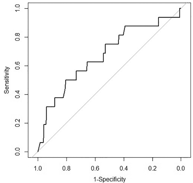
Fig. 4. AHS-4 ROC curve.
