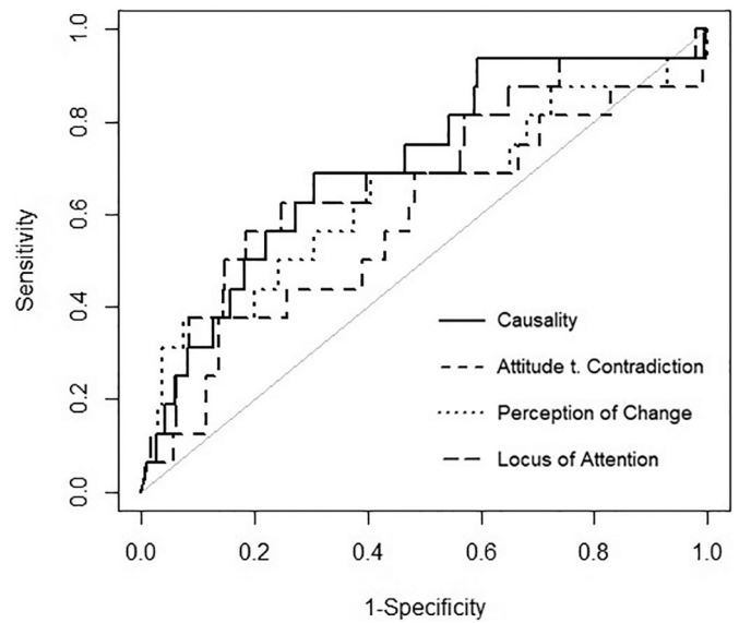
Fig. 3. AHS-12 ROC curve.
