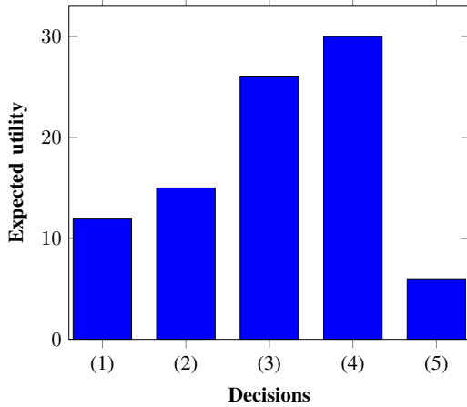
Fig. 3. A priori expected utility scores
